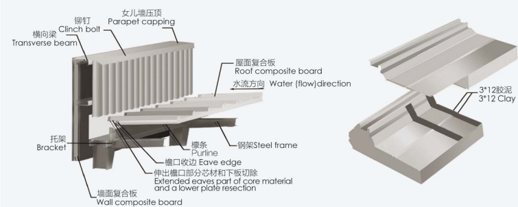
屋面檐口-III Roof eaves-III
