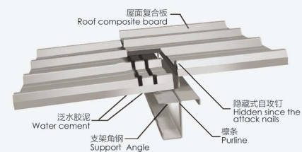
屋面板纵向搭接节点-II Roof longitudinal lap joints-II
