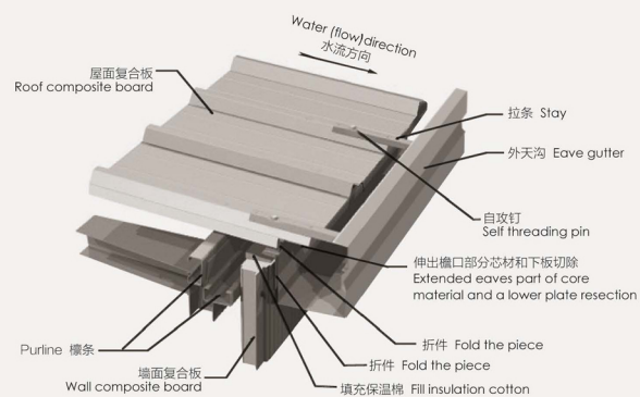
屋面檐口- II Roof eaves- II
